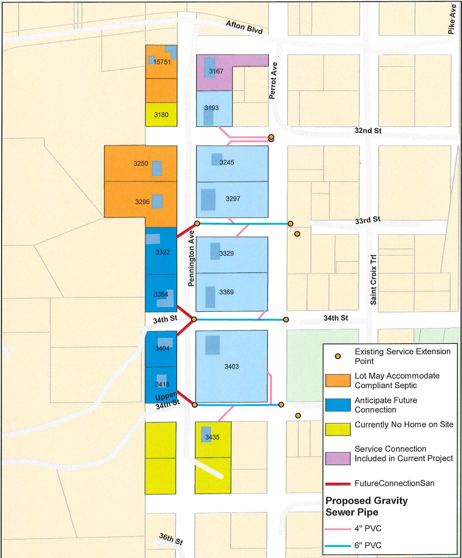
Figure 1: Pennington Sanitary Service Connection Pennington Avenue Sewer Study City of Afton
